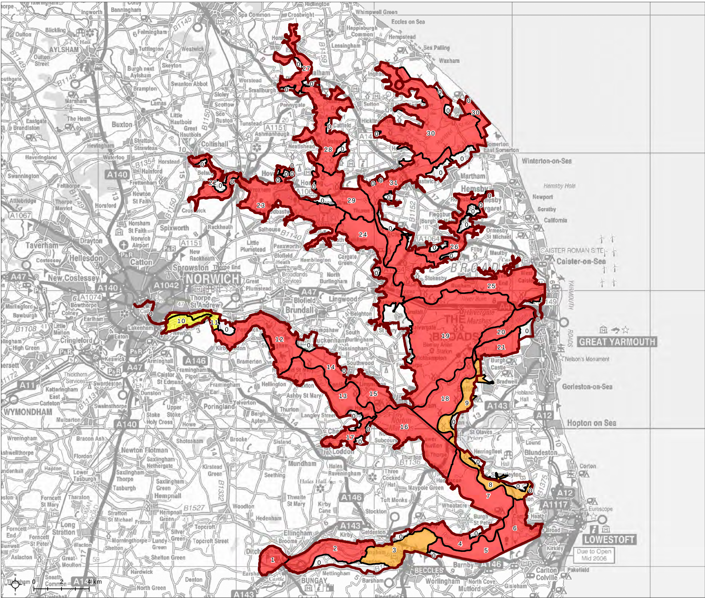
Figure 4.12 PV Sensitivity; Roof Mounted Requiring Planning Permission
