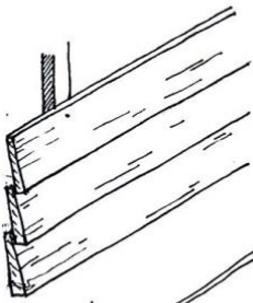
Sawn featheredge boarding. This appropriate for boathouses, boatsheds and non-residential buildings.
