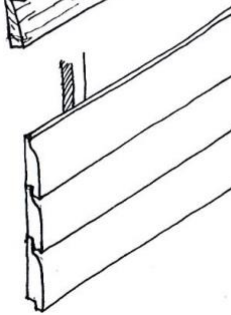
Planed shiplap boarding. This is more appropriate for residential buildings.
