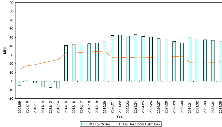
Essex Resource Zone Intermediate Framework Assessment Graph (a): Initial Solution Set & PR09 Headroom Estimates
