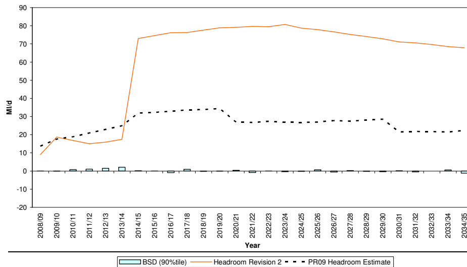
Essex Resource Zone Intermediate Framework Assessment Graph (c): Iteration 2
