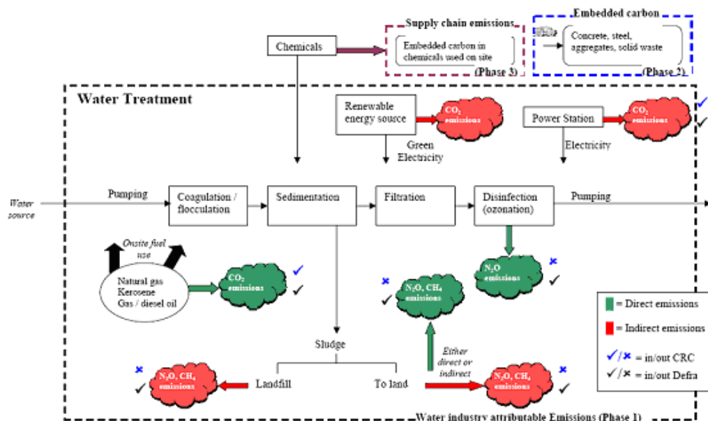
Carbon emission scope (extracted from UKWIR 2007, p.8)
