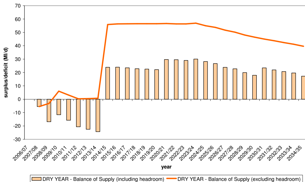
Essex Resource Zone - Balance of Supply for Final Planning Dry Year Scenario
