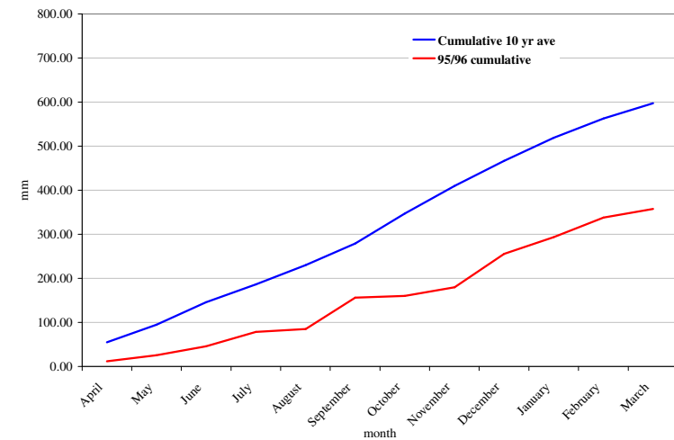
Cumulative monthly rainfall vs cumulative 10 year LTA monthly rainfall 95/96
