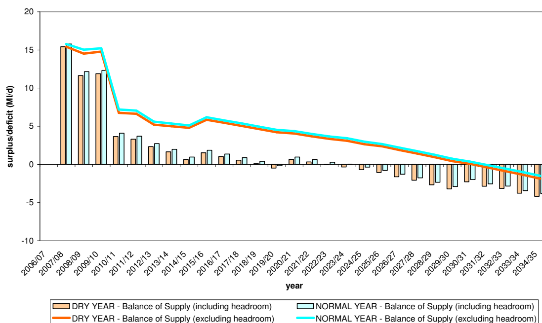
Suffolk Northern/Central Resource Zone - Balance of Supply for Baseline Dry and Normal Year Planning Scenarios
