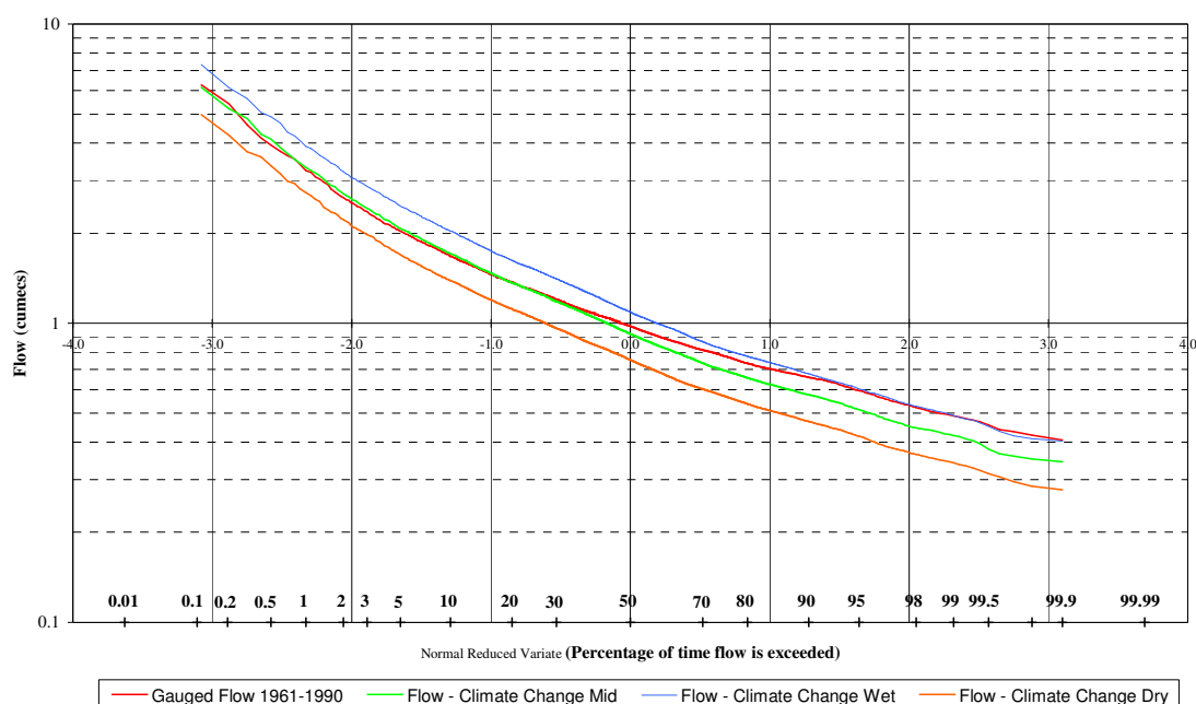
Figure 3: Flow Duration Curve for River Bure @ Ingworth
