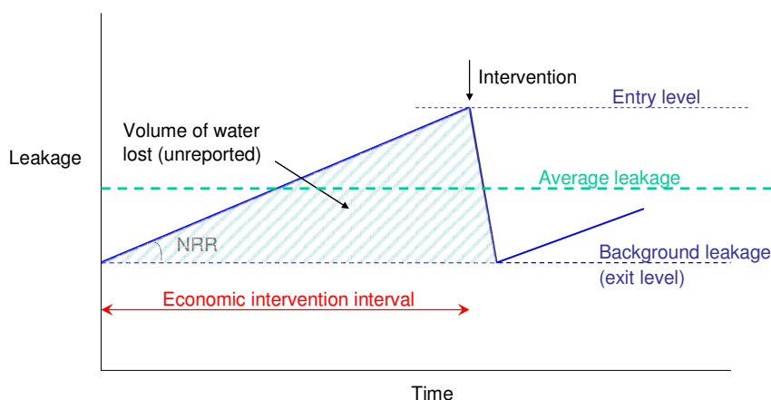
Figure 5.4.2 Hypothetical profile of leakage in a DMA
